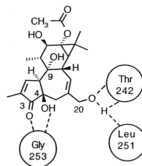
FIGURE 4. Hydrogen bond networks of the phorbol/PK-Cδ C1b complex.
